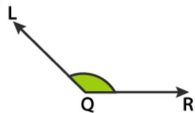
Obtuse angle \angle LQR
